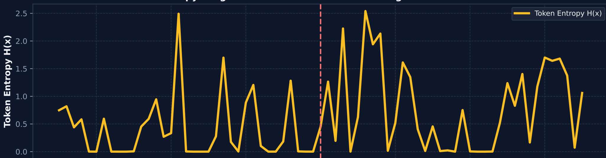
Panel B: Real Shannon Entropy Surge Around Exact Second-Guessing Point
