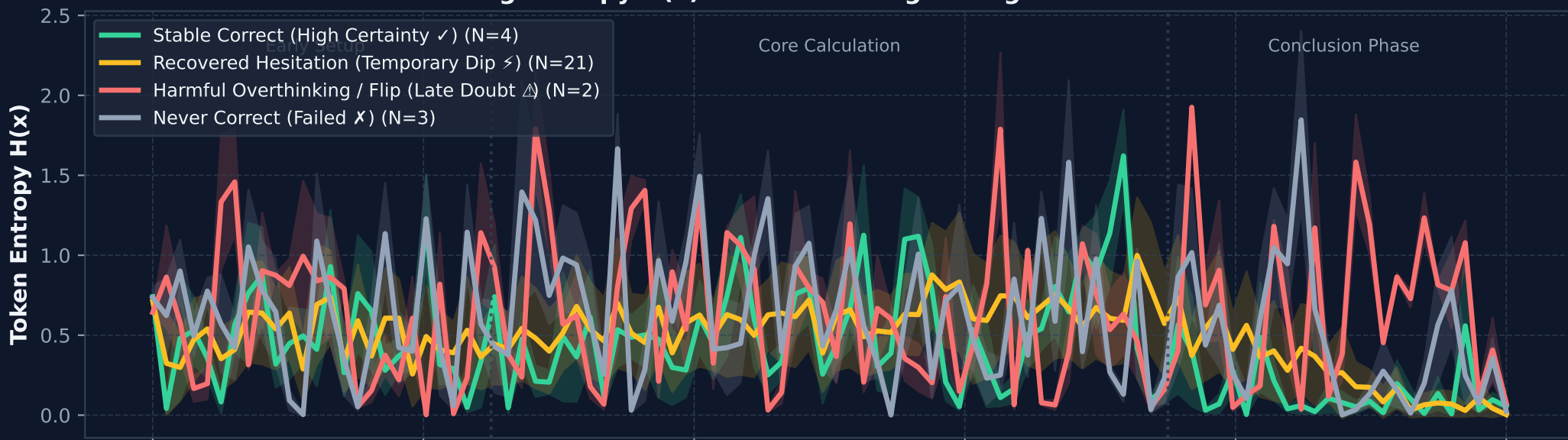
Panel B: Confidence Separation — Collapse During Harmful Overthinking
