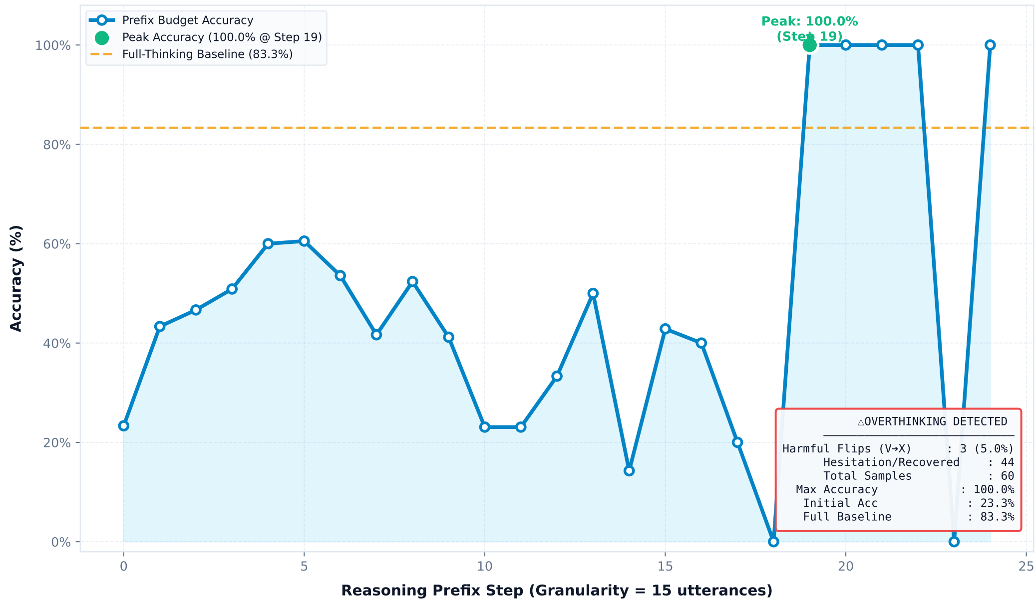
Panel A: Accuracy Progression vs. Thinking Step (r1_distill_qwen1_5b on gsm8k)
