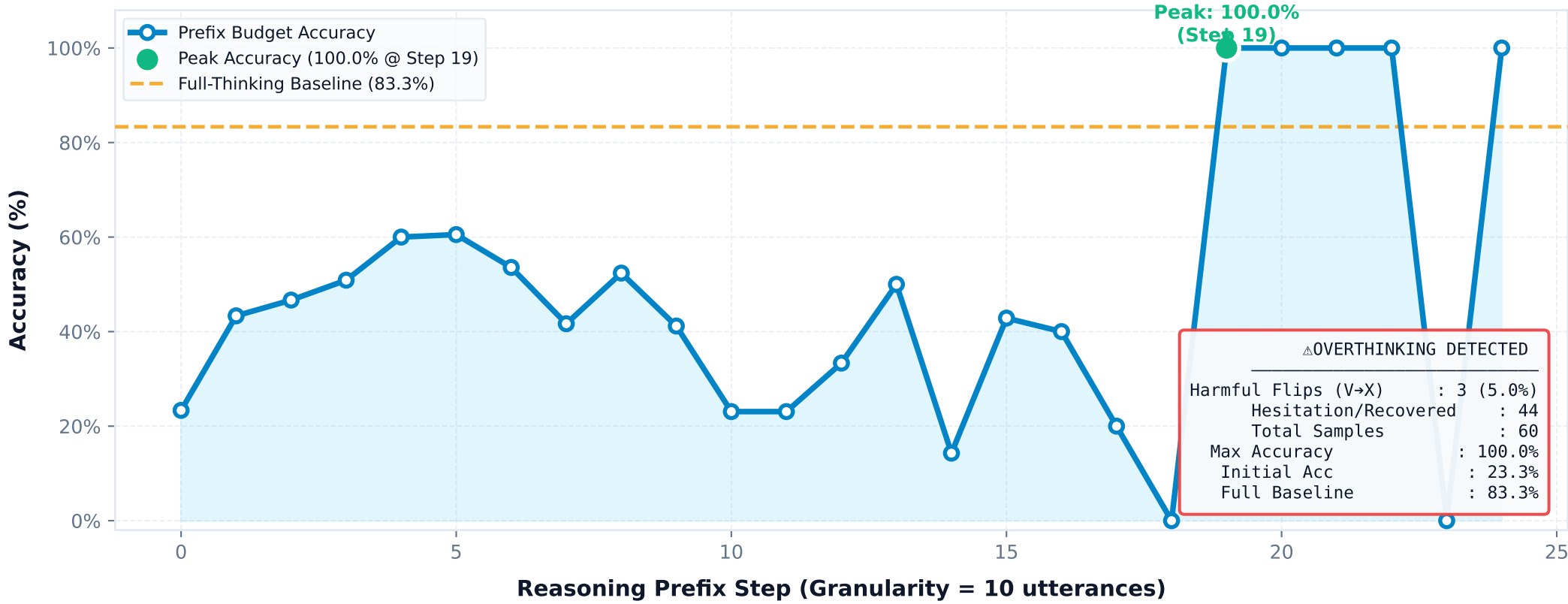
Panel A: Accuracy Progression vs. Thinking Step
