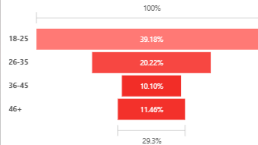
Attrition Rate by Age Group
