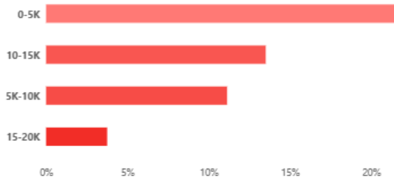
Attrition Rate by Income Range
