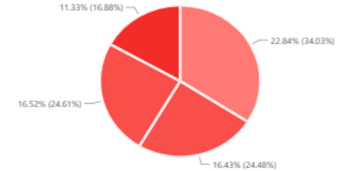
Attrition Rate by JobSatisfaction
