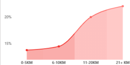
Attrition Rate by Distance From Home
