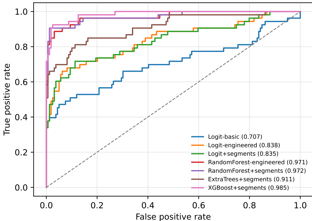
ROC curves on held-out travelers
