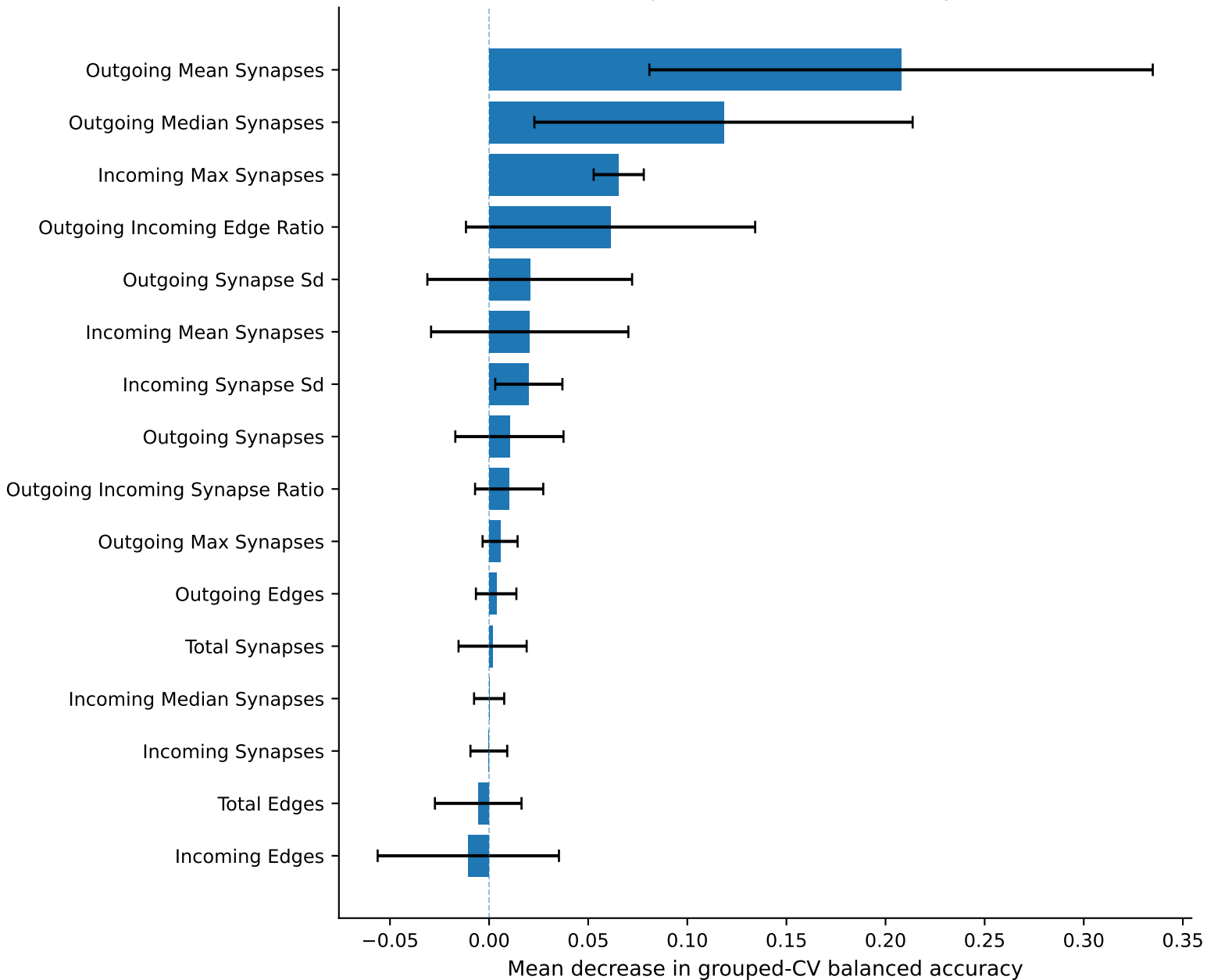
Permutation Importance of Connectivity Features
