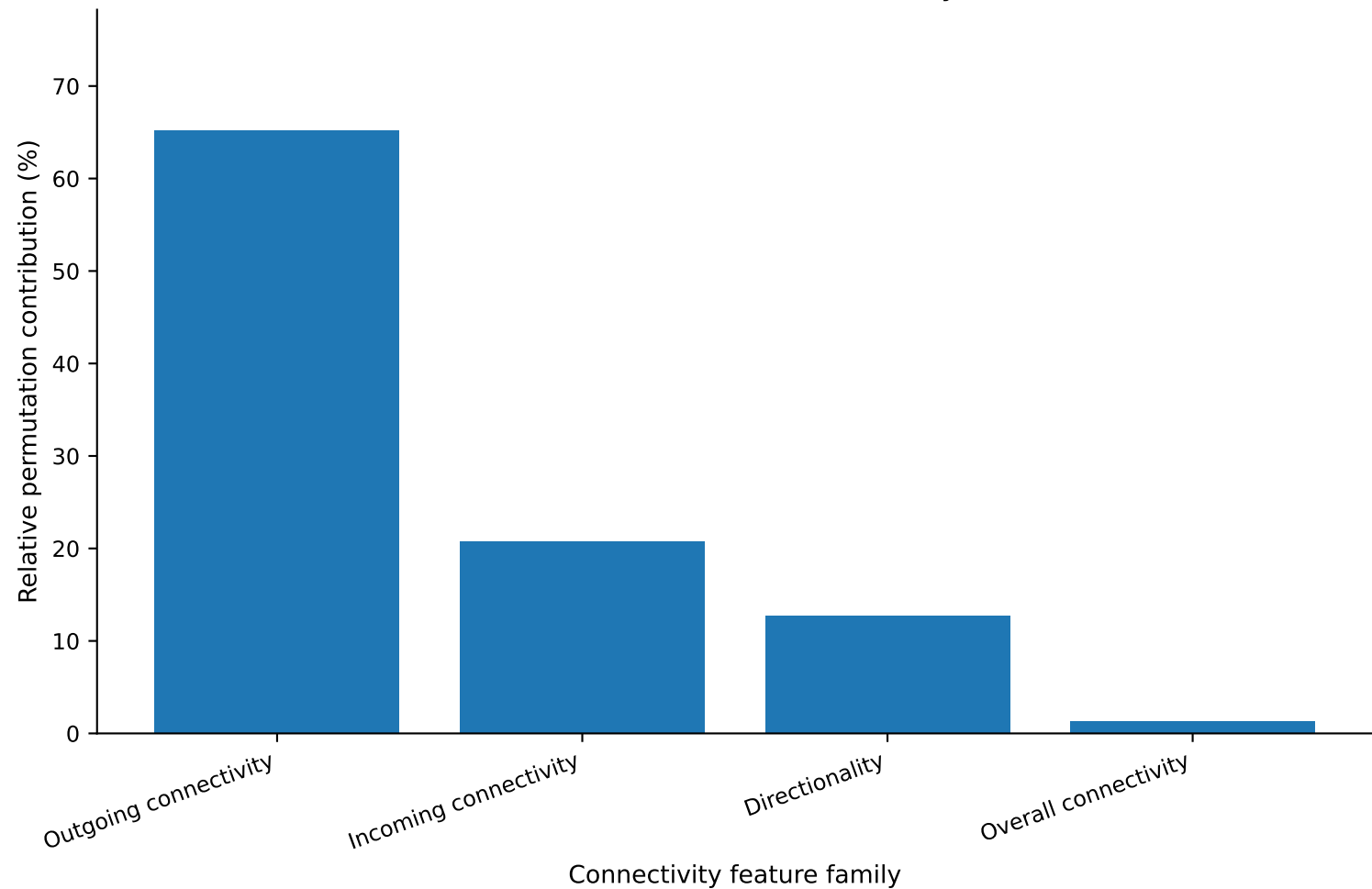
Relative Predictive Contribution of Connectivity Feature Families
