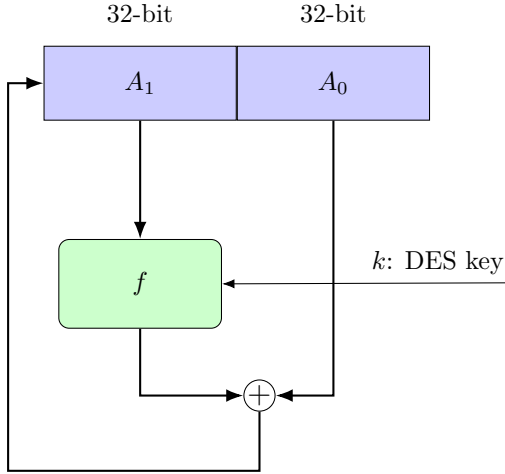
Figure 5: Shift register within Minipage
