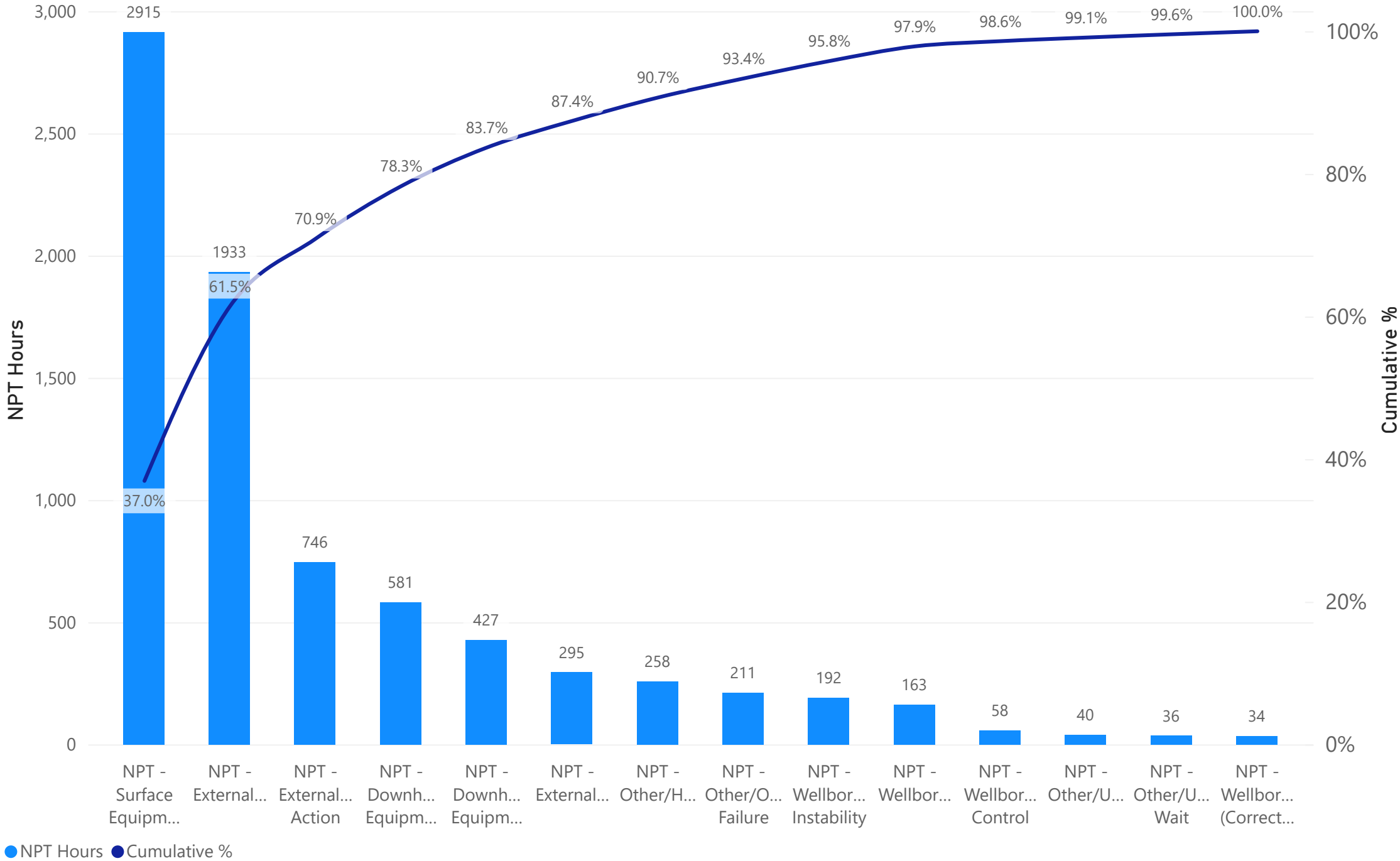
NPT Hours by Category and Cumulative %
