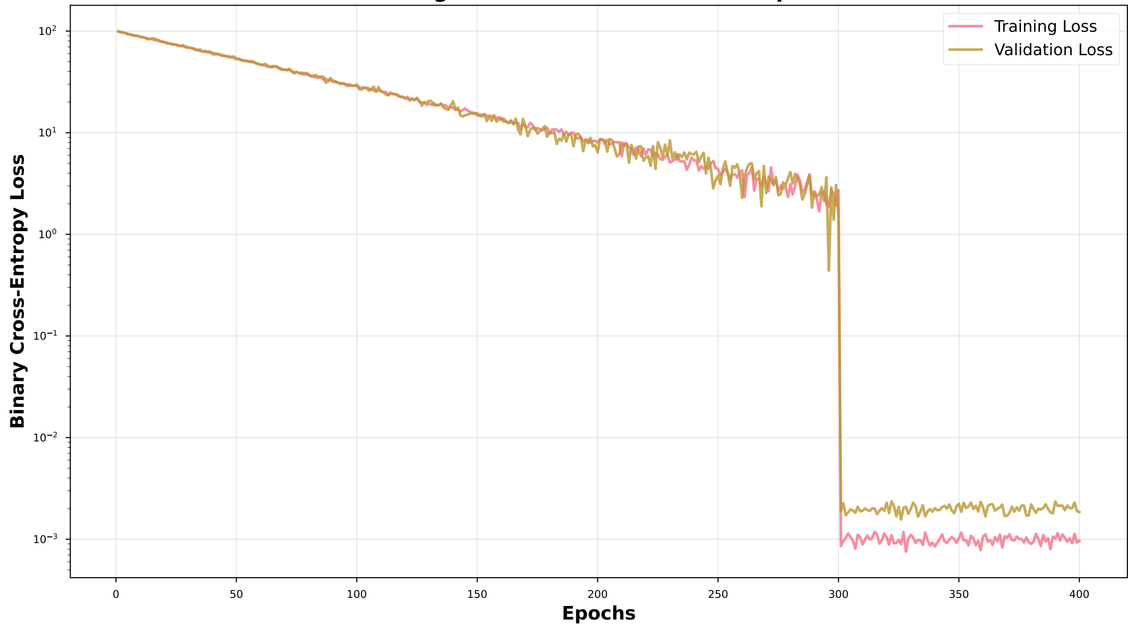
Training and Validation Loss Over Epochs
