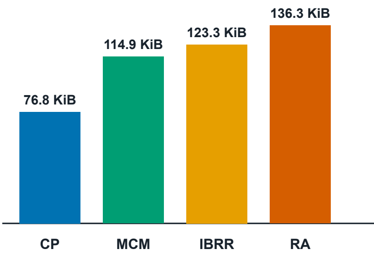
C. Proof size
