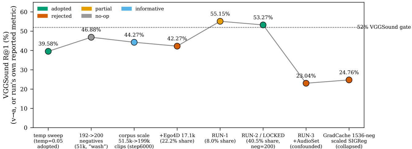
M2 experimental chronology — 8 decision points (of 36 total runs; see METHODOLOGY_FORENSICS.md §1.1 for the full run table)
