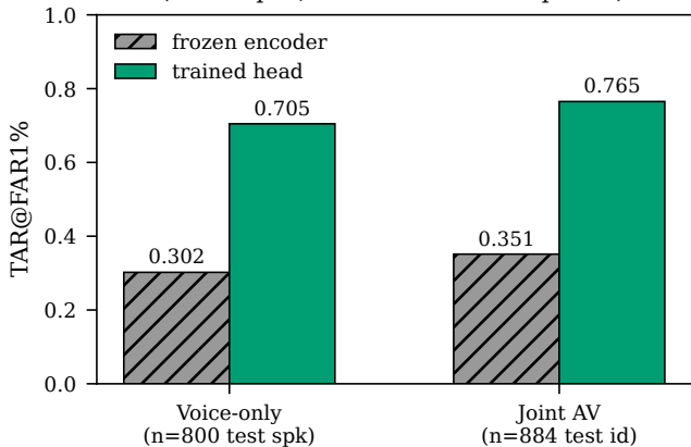
Identity head: frozen encoder vs. trained head (full-corpus, current-best checkpoints)
