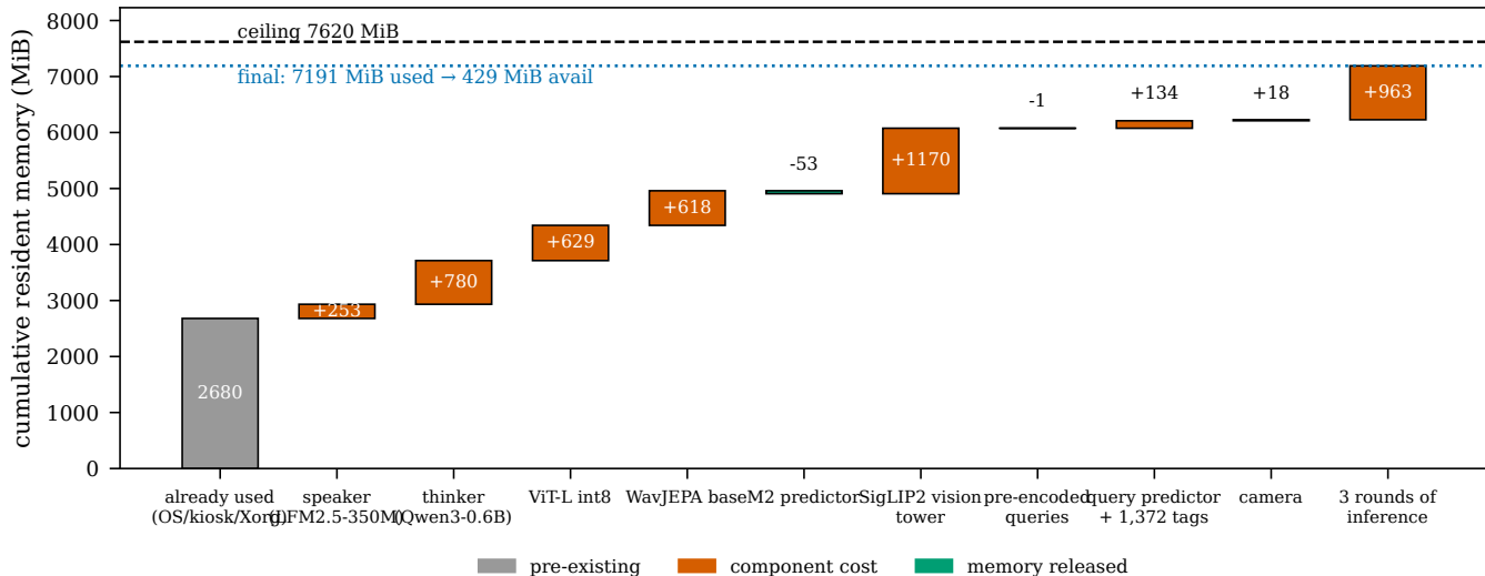
Jetson memory waterfall, current (no-nat) production stack, MAXN_SUPER (ARCHITECTURE.md §8.1, 2026-08-15)
