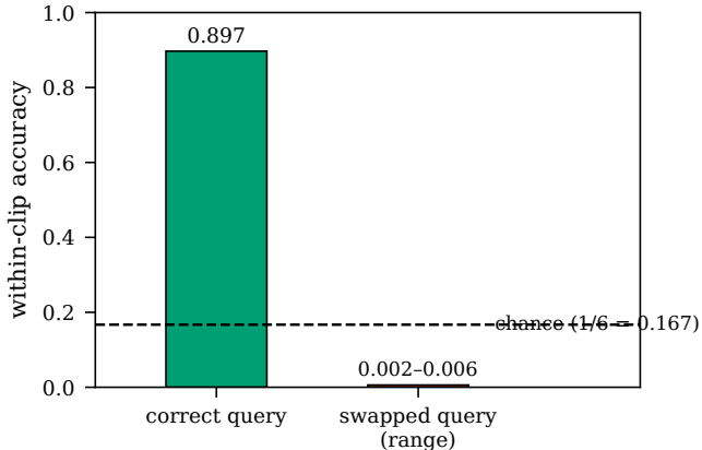
Query predictor swapped-query control
