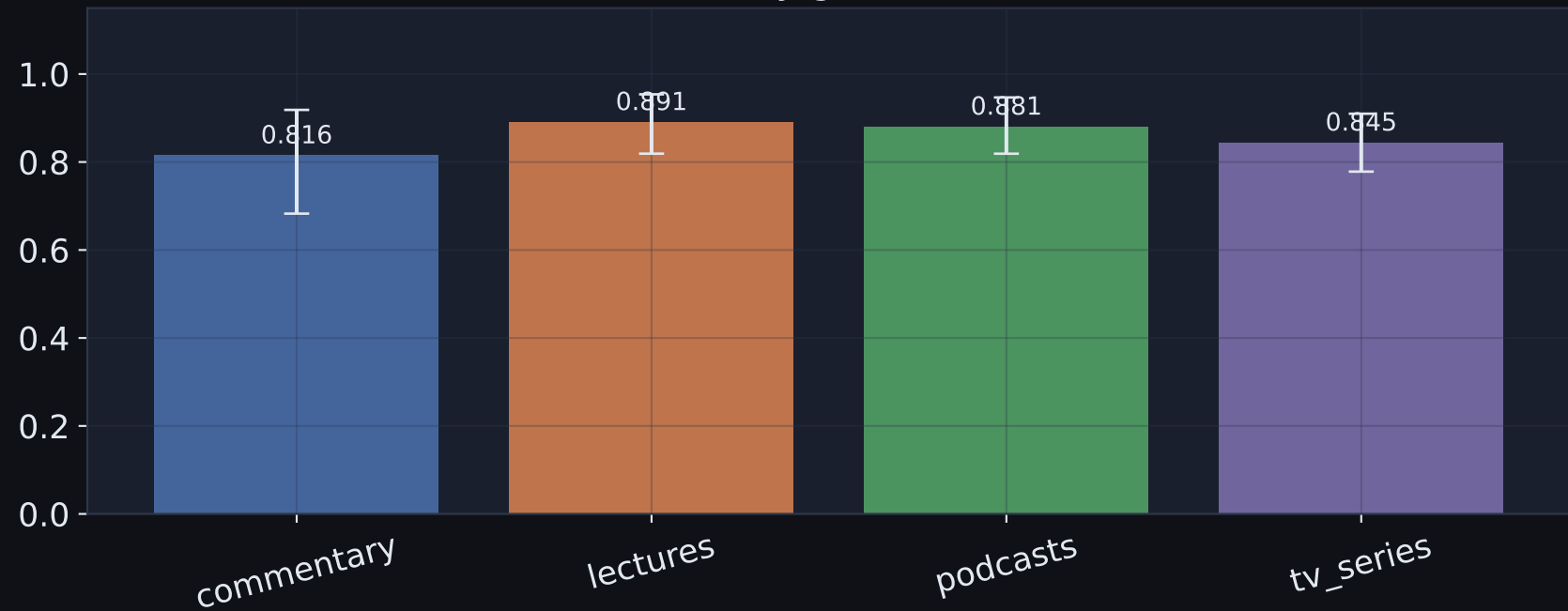
AUC-ROC by genre (95% CI)
