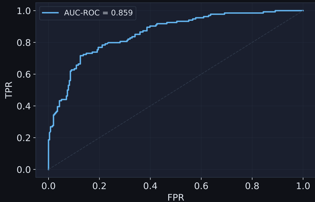
ROC curve
