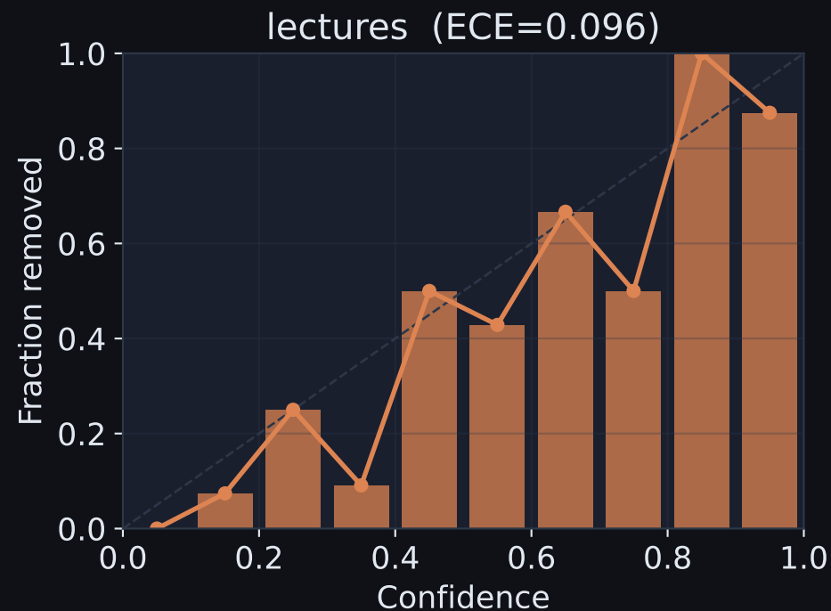
Calibration varies by genre — panels show fraction removed vs confidence
