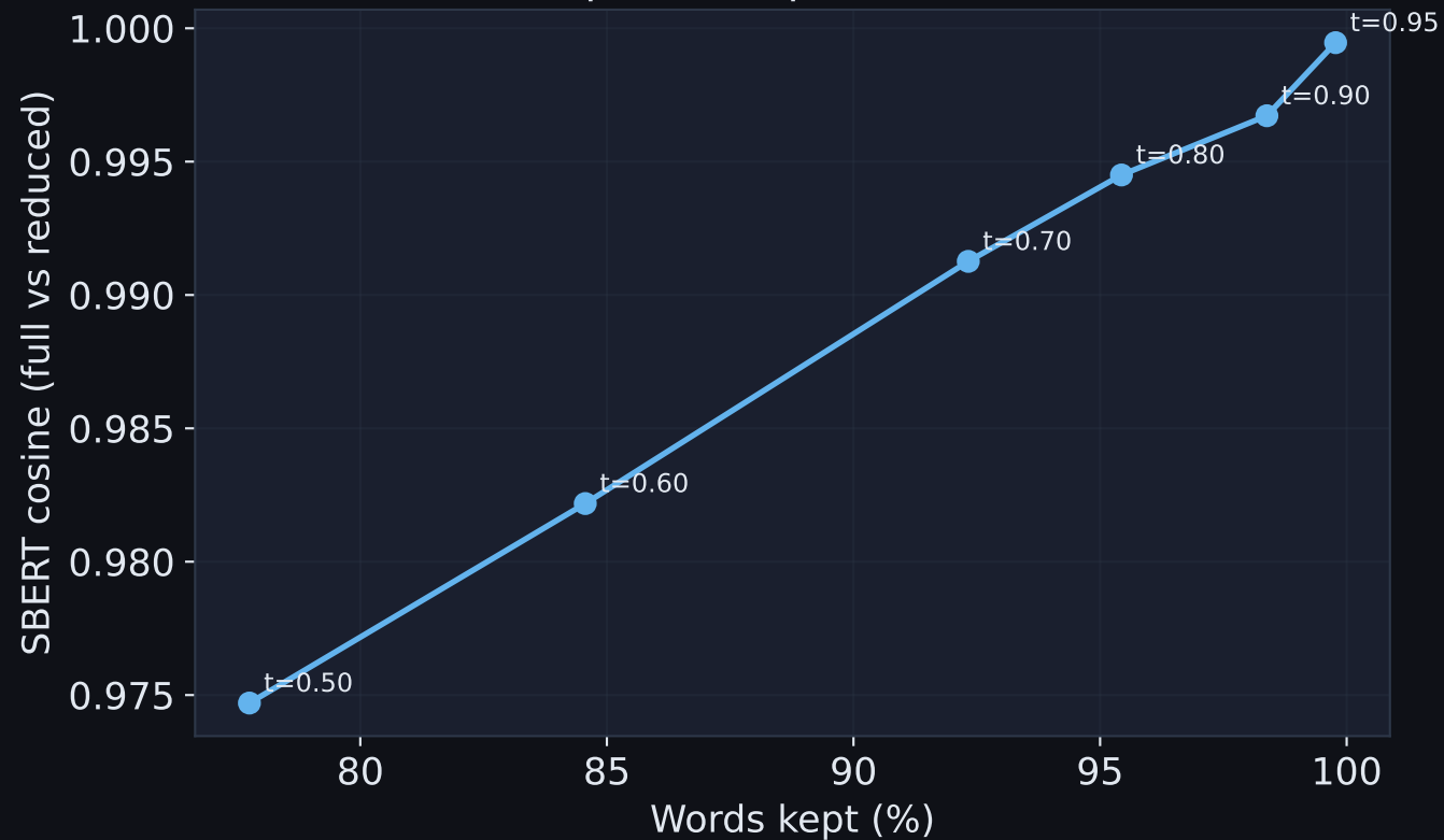
Overall compression-preservation trade-off
