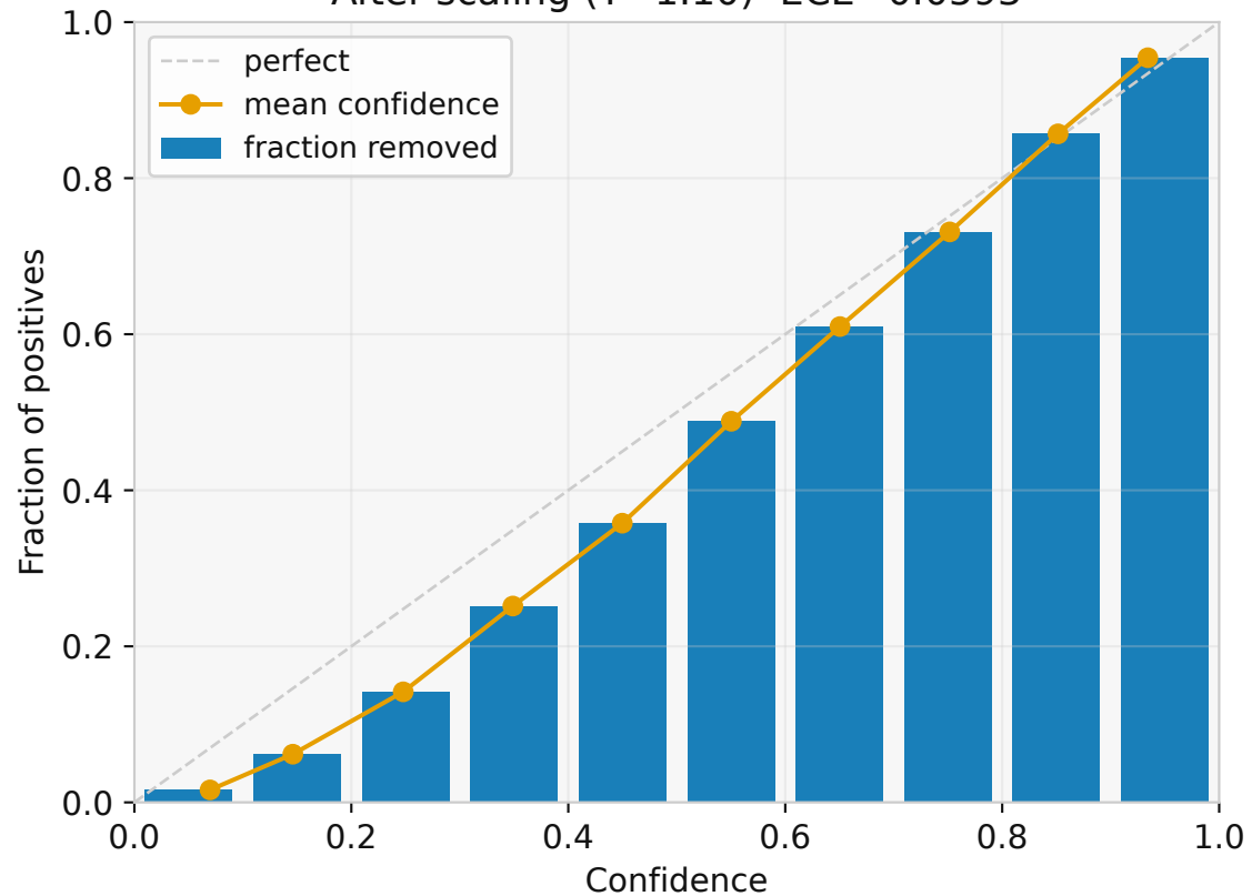
After scaling ( T=1.10 ) ECE=0.0593
