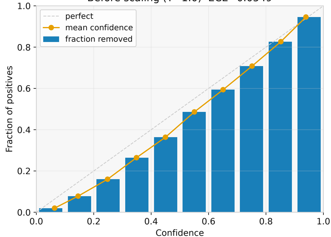
Before scaling ( T=1.0 ) ECE=0.0549
