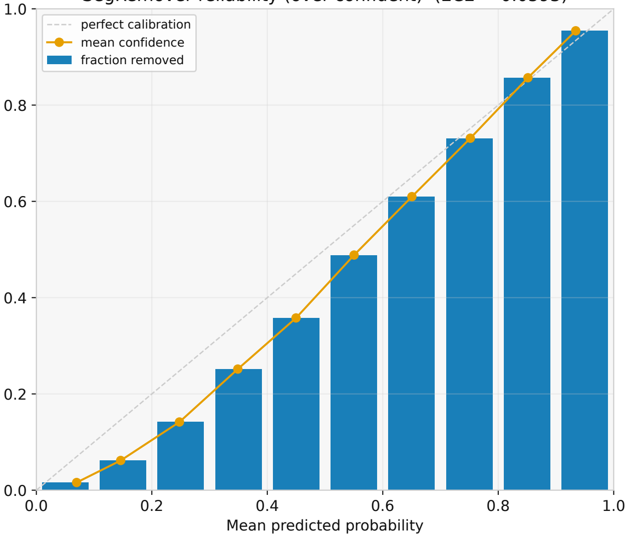
SegRemover reliability (over-confident) (ECE = 0.0593)
