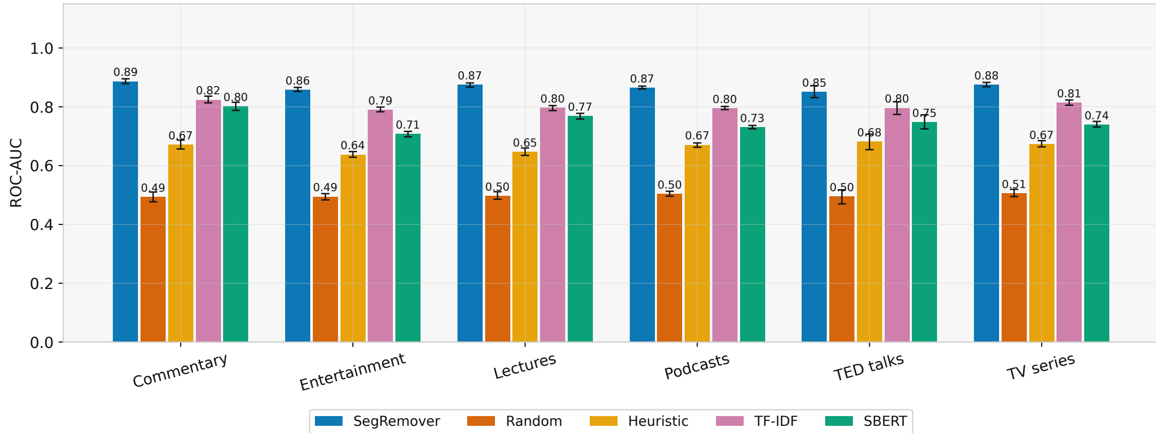
SegRemover advantage over baselines varies by genre
