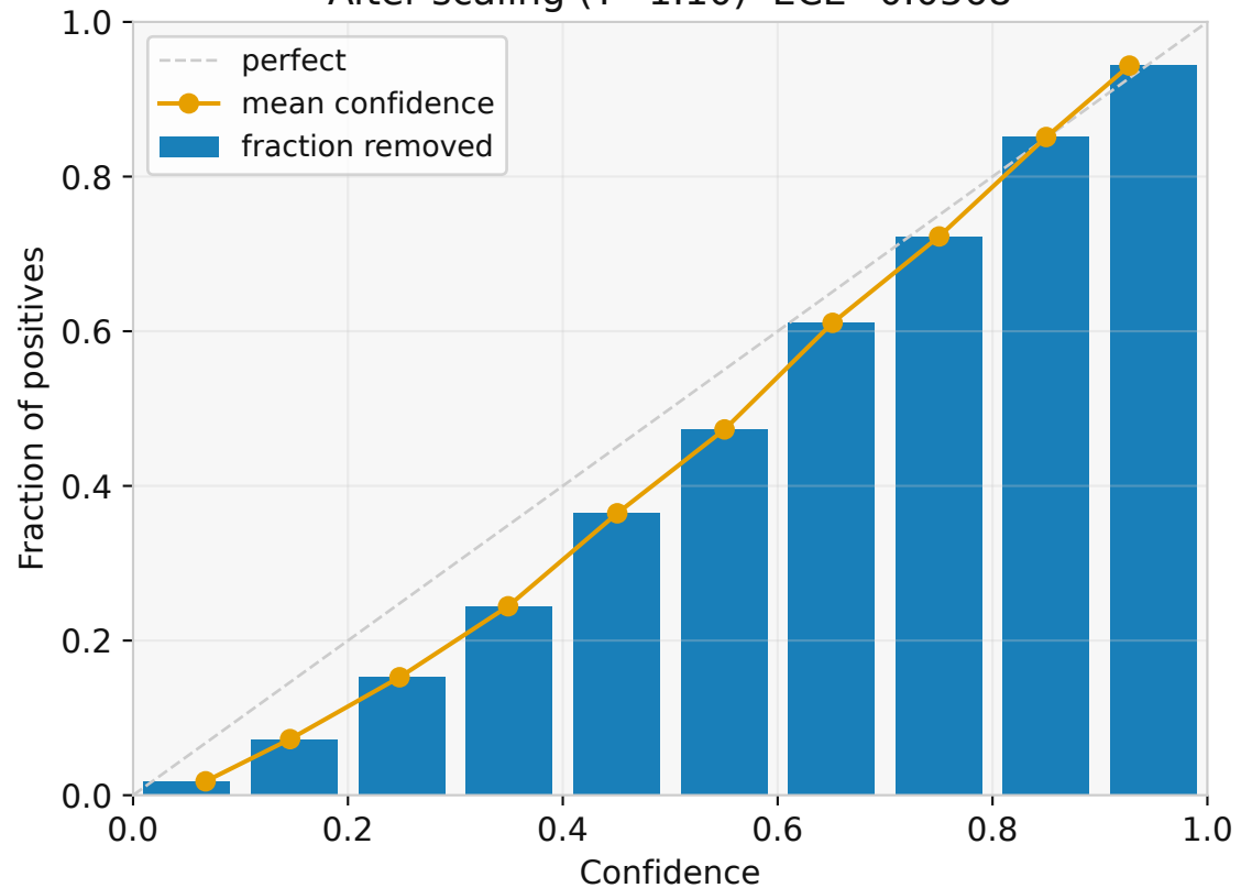
After scaling (T=1.10) ECE=0.0568
