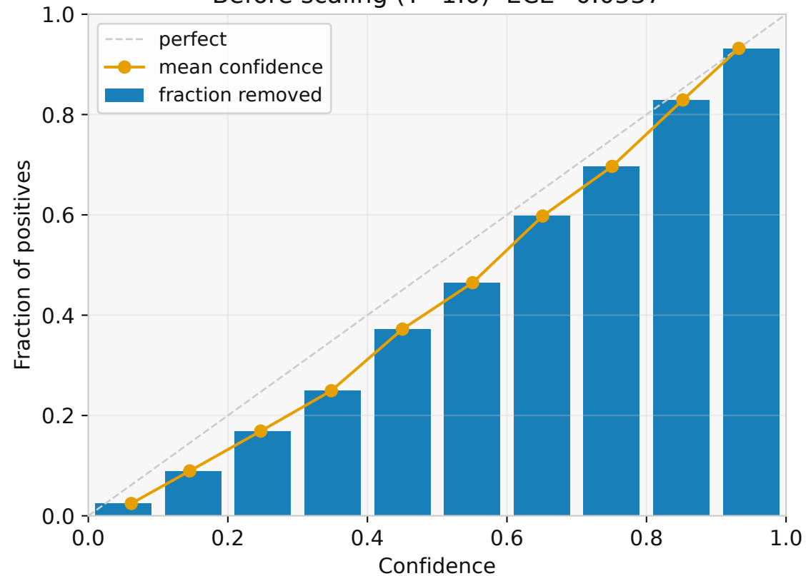
Before scaling (T=1.0) ECE=0.0537
