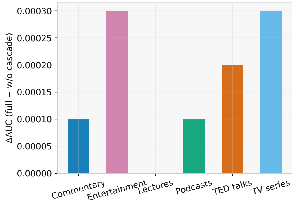
(a) \Delta\text{AUC} per genre
