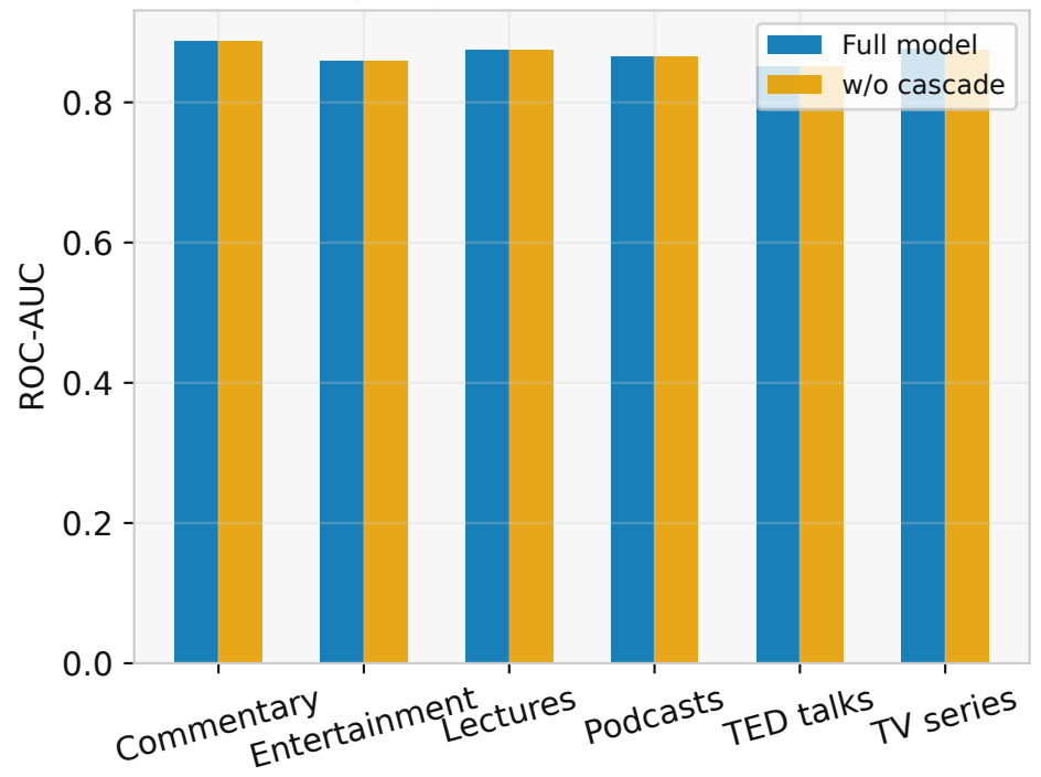
(b) ROC-AUC per genre: full model vs. w/o cascade
