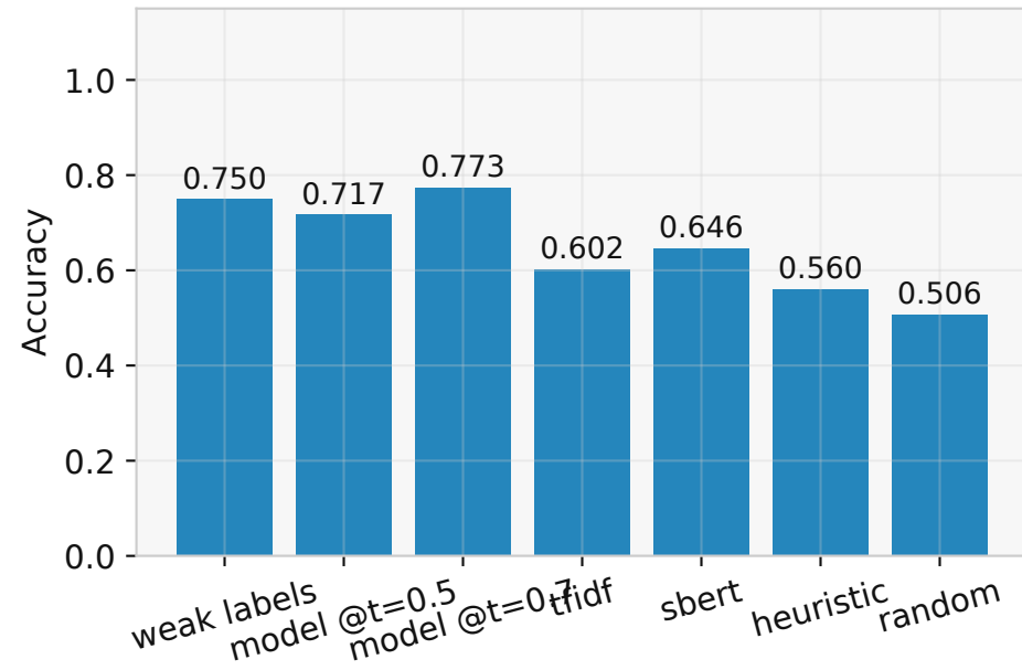
Accuracy
