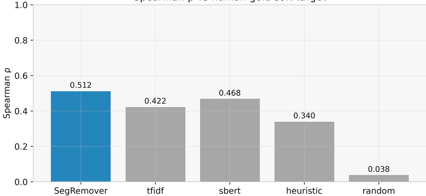
Spearman \rho vs human gold soft target
