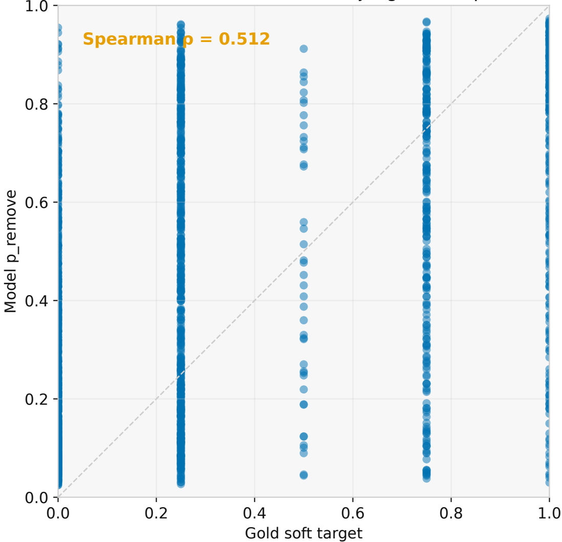
Model rank correlates with human judgement ( \rho=0.512 )
