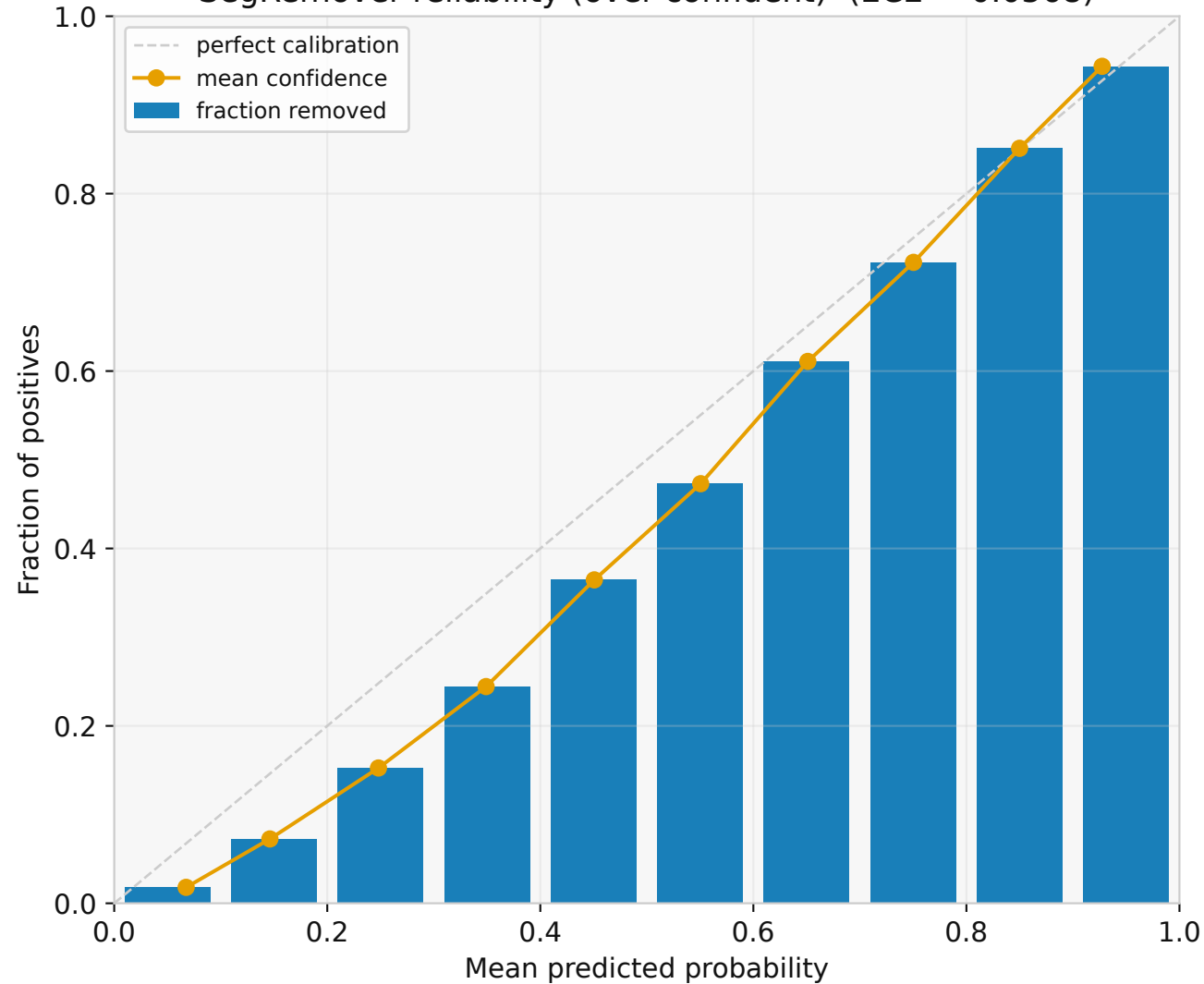
SegRemover reliability (over-confident) (ECE = 0.0568)
