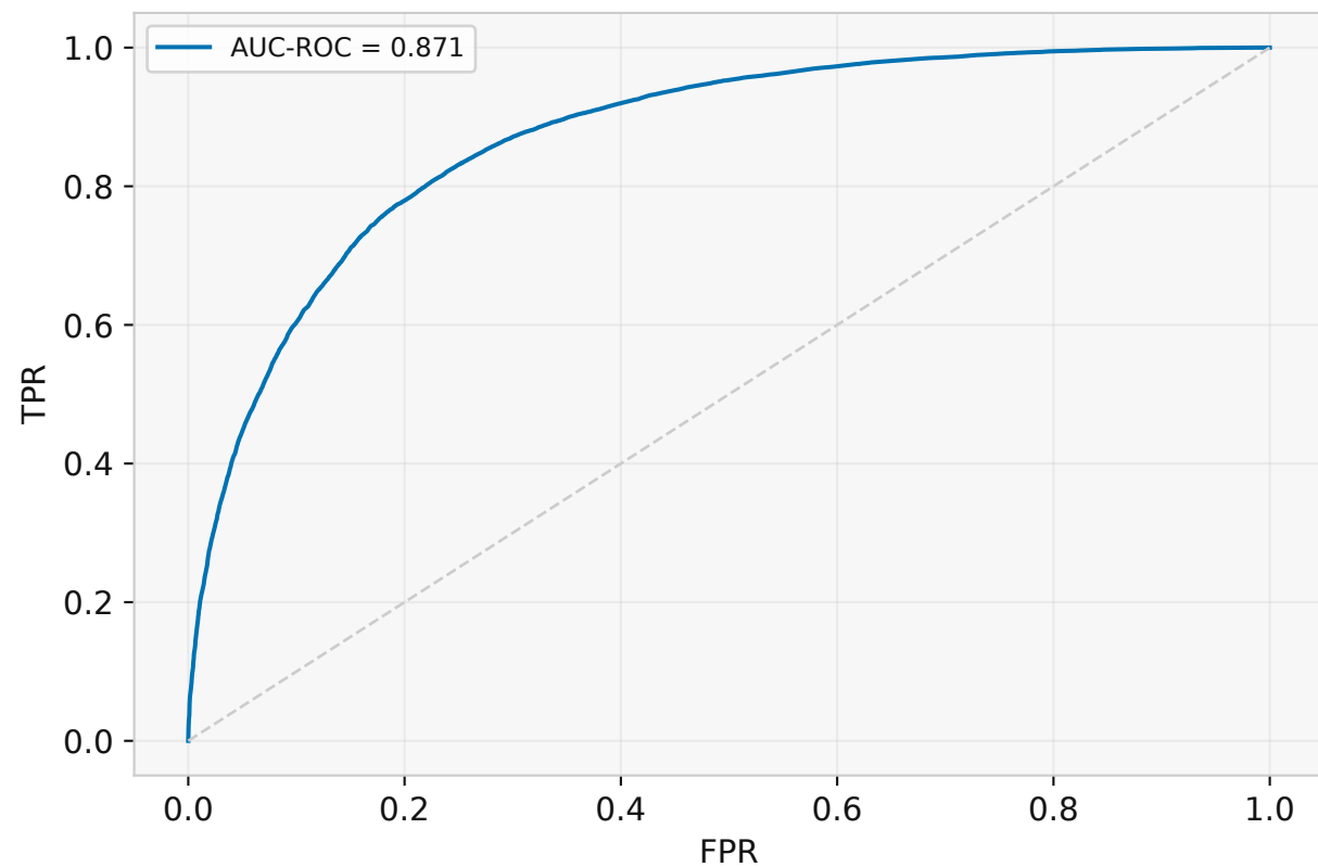
ROC curve
