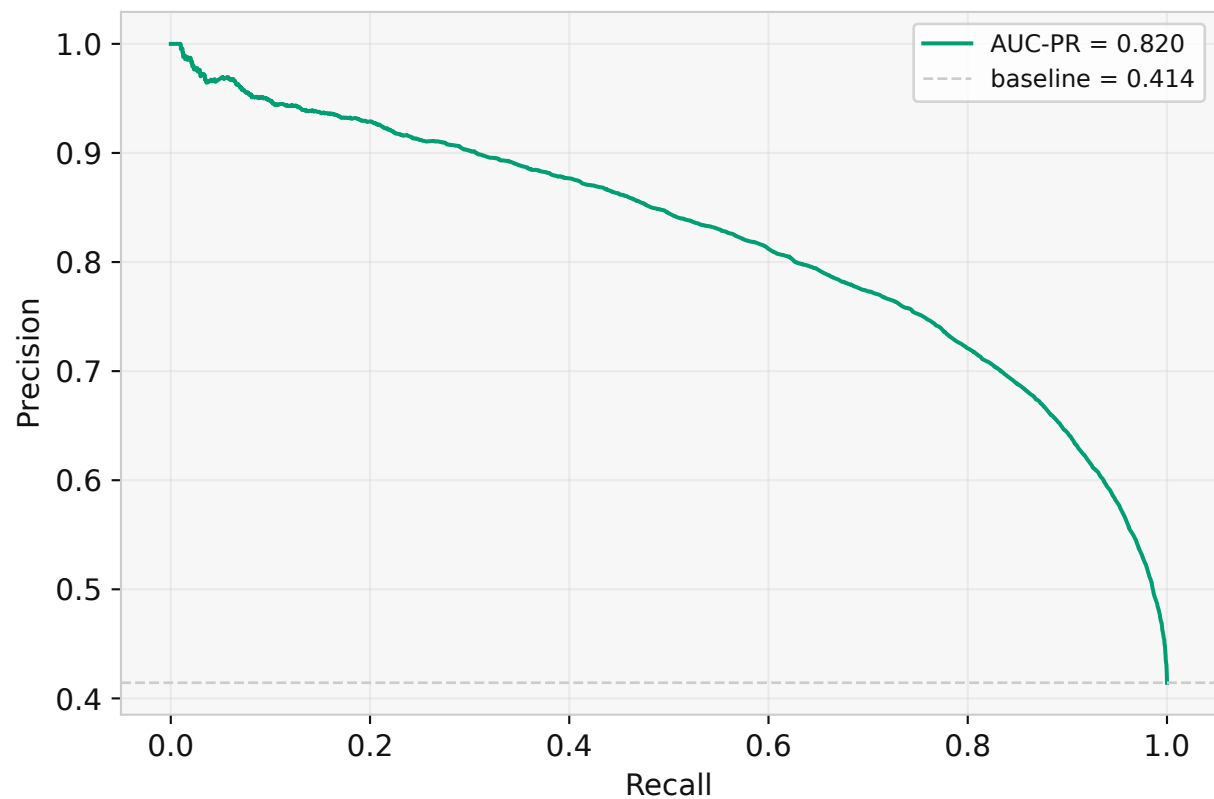
PR curve
