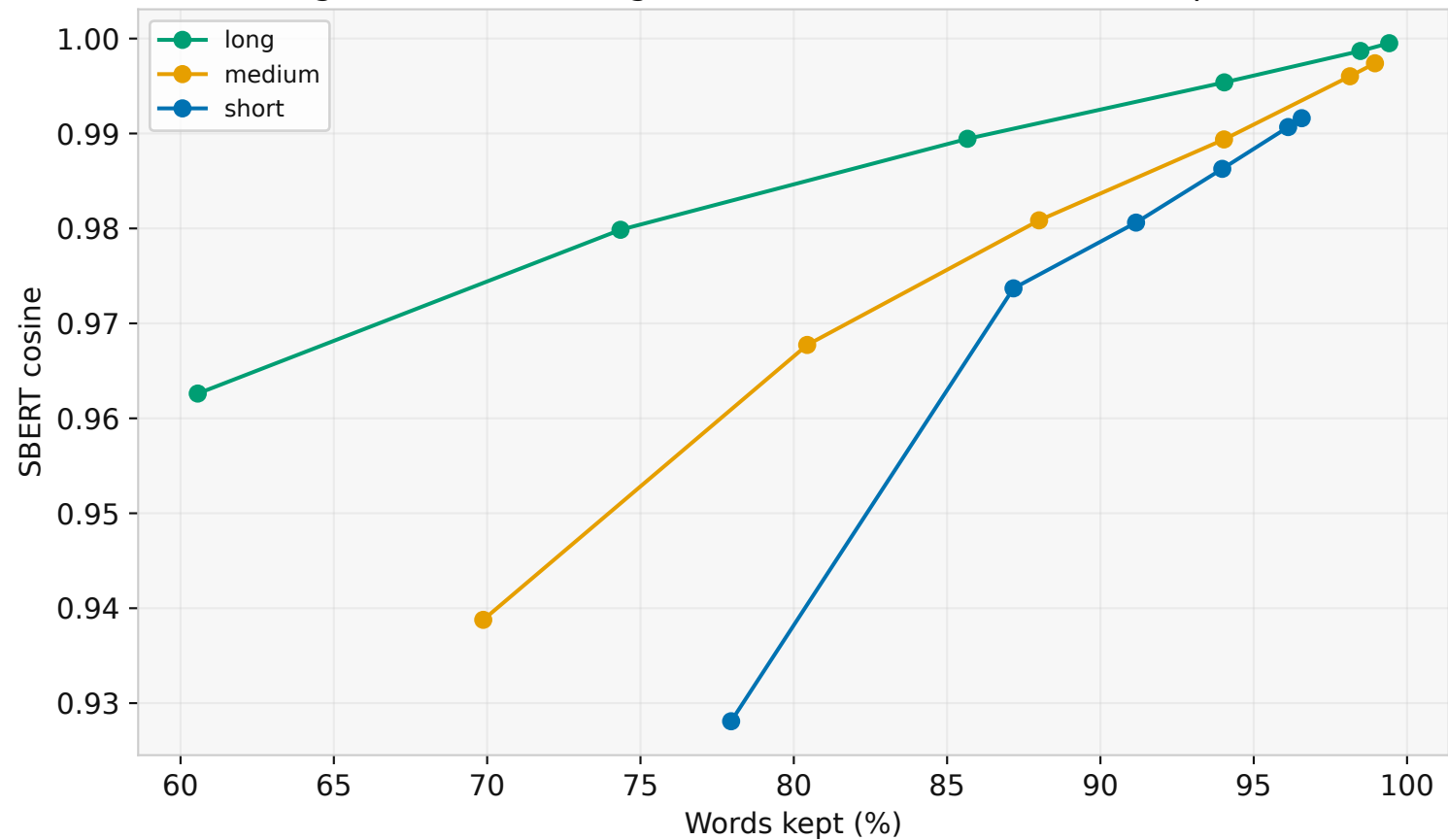
Longer videos show higher semantic robustness to compression
