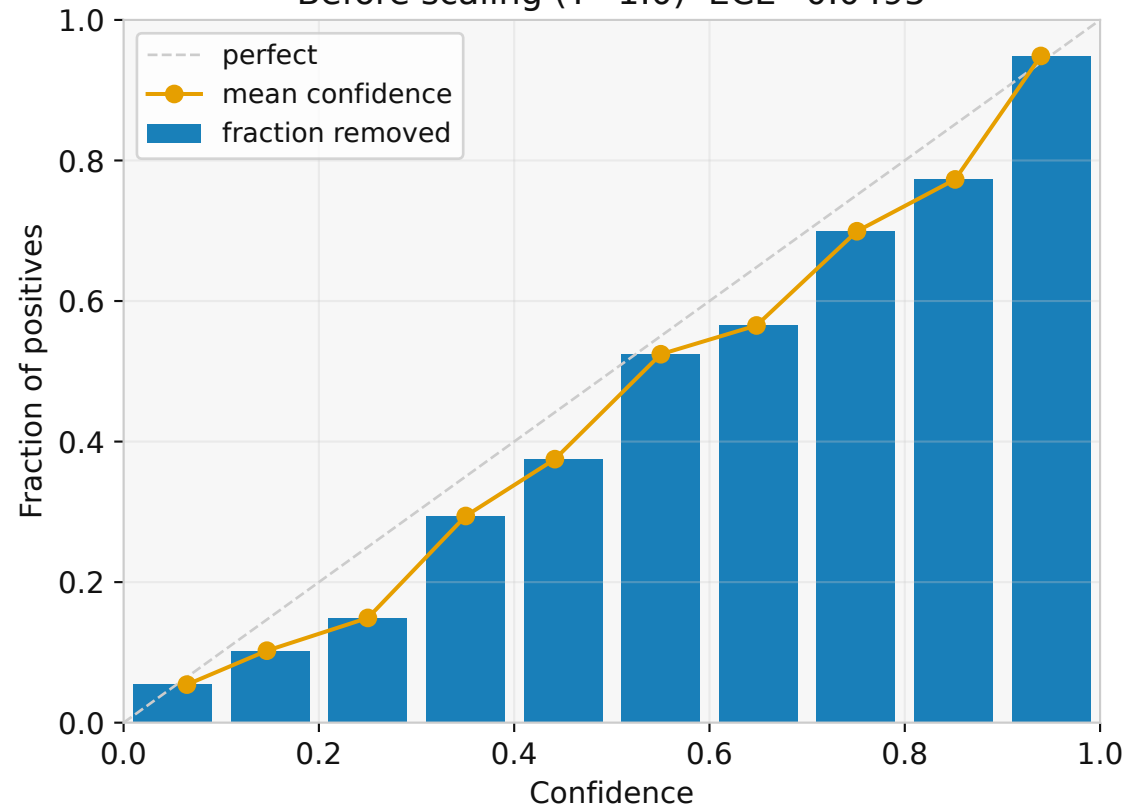
Before scaling ( T=1.0 ) ECE=0.0495
