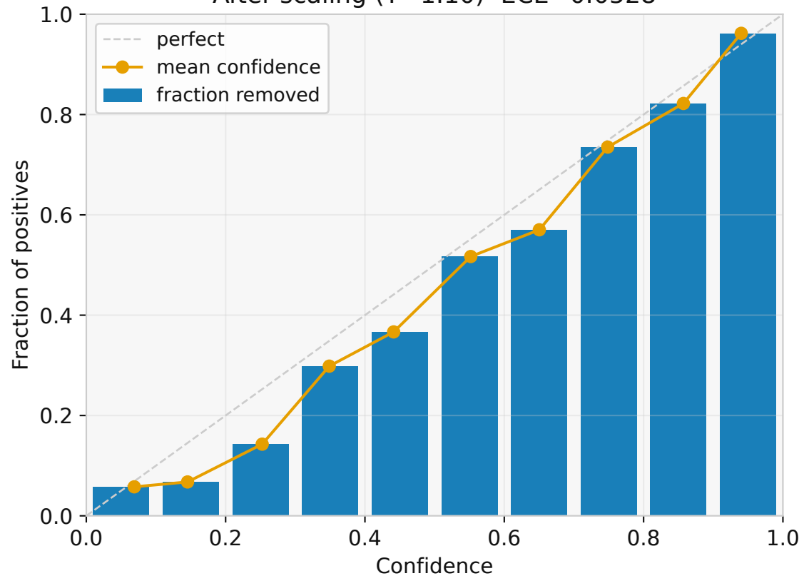
After scaling ( T=1.10 ) ECE=0.0528
