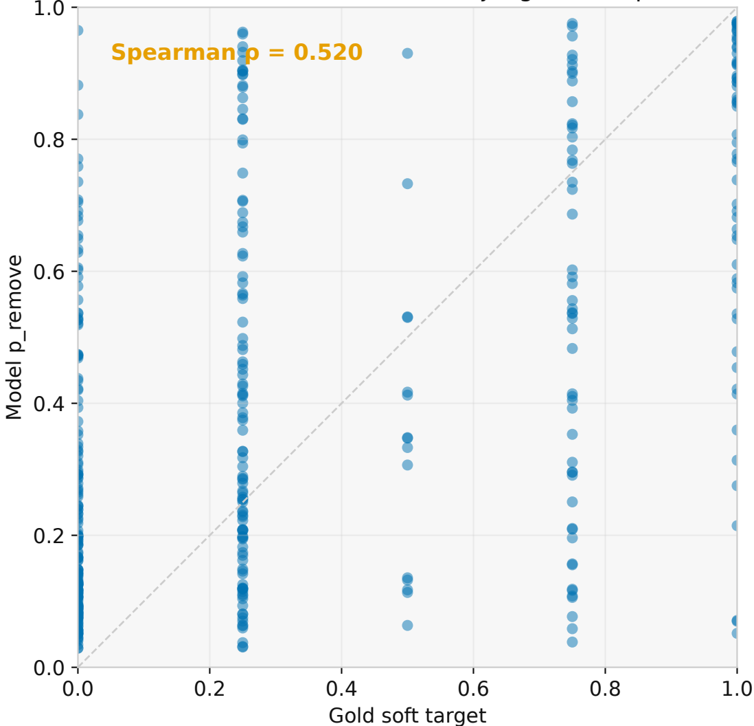
Model rank correlates with human judgement ( \rho=0.520 )
