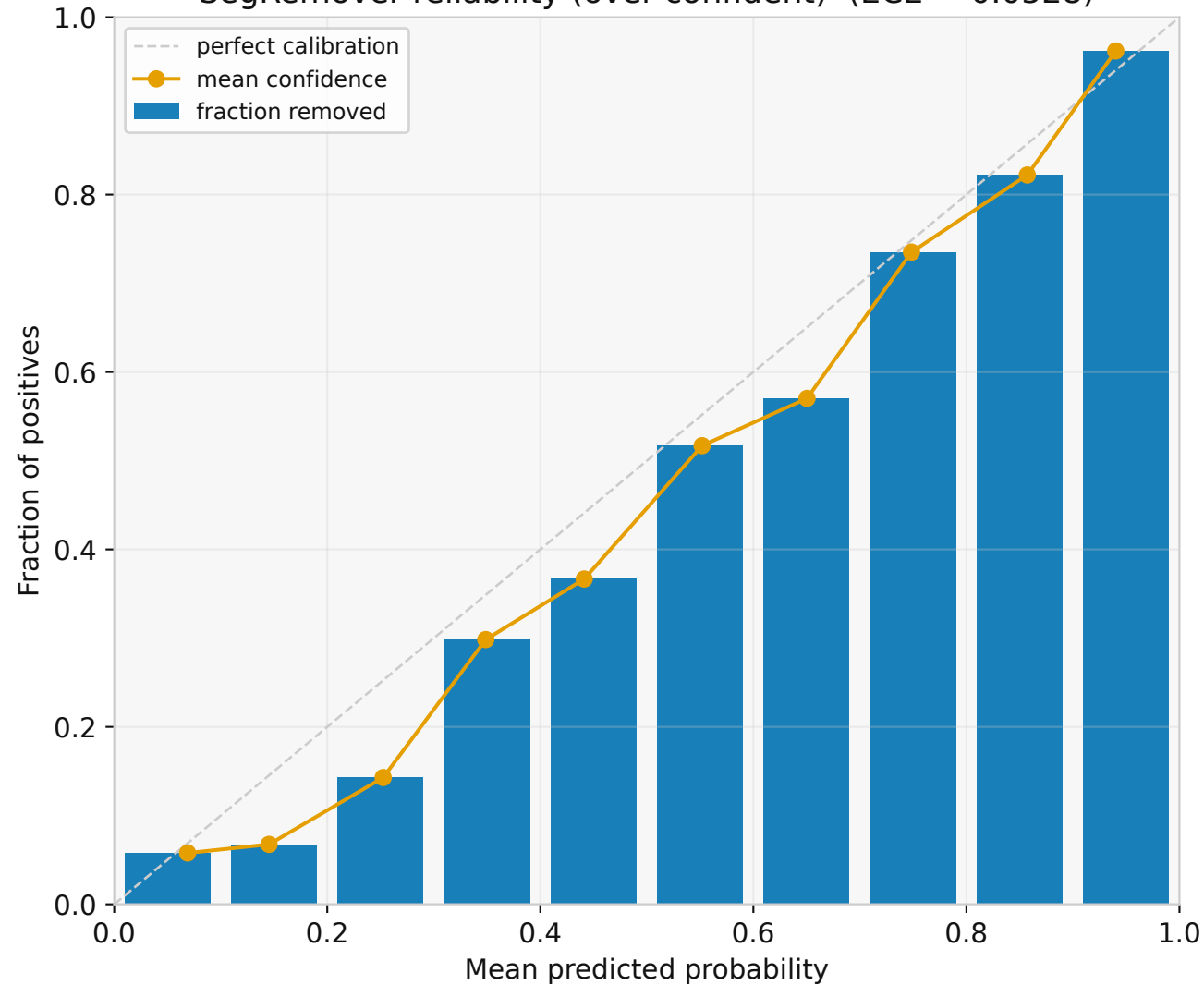
SegRemover reliability (over-confident) (ECE = 0.0528)
