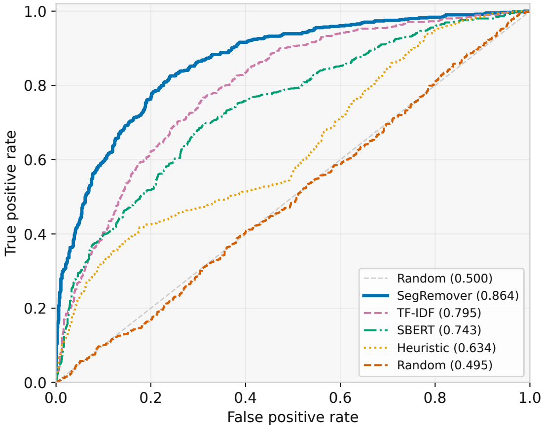
ROC curves — SegRemover vs baselines
