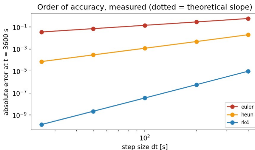
Figure. Error after one hour against the step size, on logarithmic axes. The slopes of the three lines are the orders of the methods. The five points of each line belong to the steps 25, 50, 100, 200 and 400 s, and the dotted lines of the exact slopes 1, 2 and 4 lie hidden under the measured lines.
