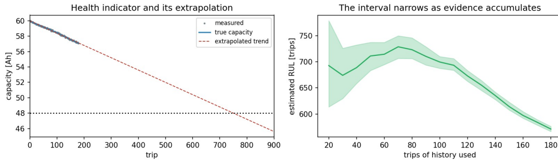
Figure. Left: The measured capacity of 180 trips with the fitted line, extended to the end-of-life level of 48 Ah (dotted). Right: The estimated remaining useful life (RUL) and its 90 percent interval against the number of trips of history used.
