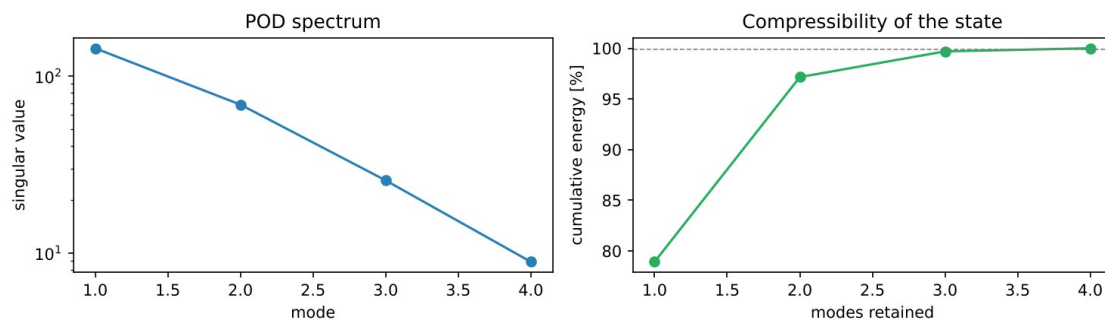
Figure. Left: The four singular values of the snapshots of the pack model, the spectrum of the proper orthogonal decomposition (POD). Right: The cumulative energy of the modes. Two modes carry about 97 percent, of a four-state system.
