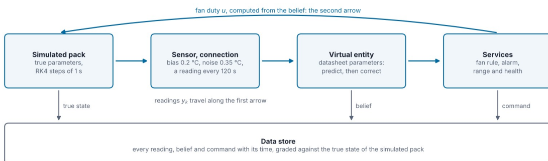
The twin of the pack after Day 1: one loop of five parts, once per simulated second
