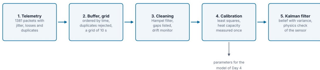
The twin of the pack after Day 3: from packets to a calibrated, filtered belief
