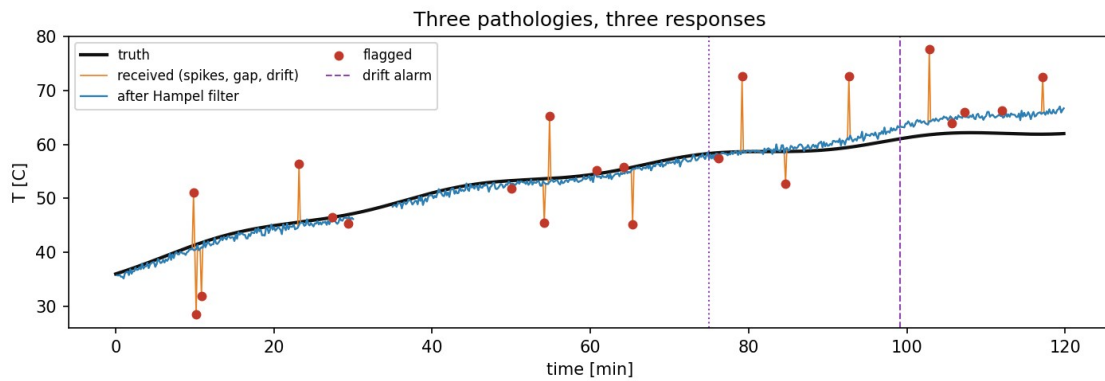
Figure. The telemetry of the pack over two hours with its spikes, its gap and its drift. The dotted line marks the start of the drift and the dashed line the drift alarm.
