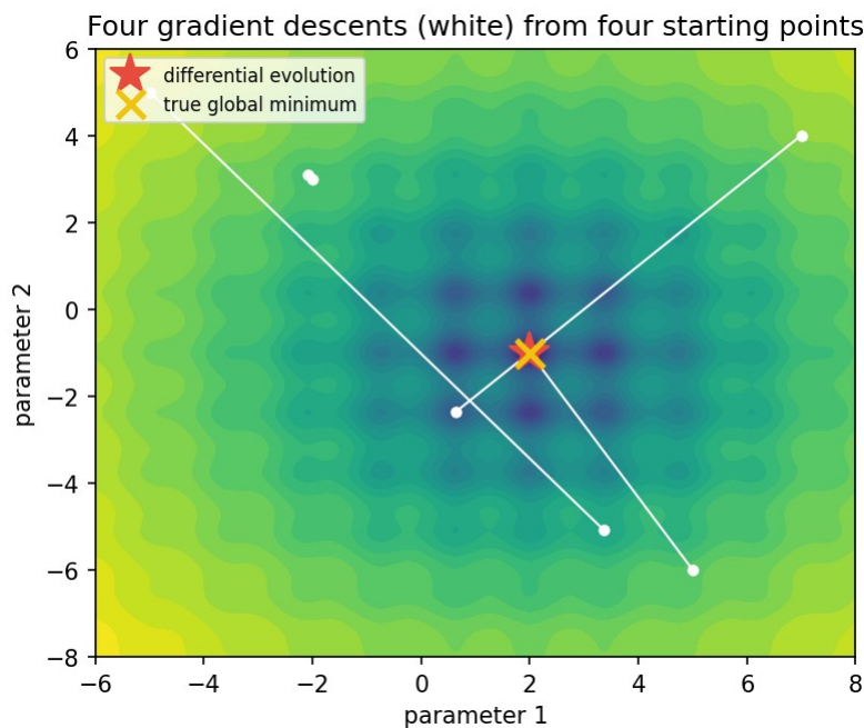
Figure. The rugged test function, dark for low values. Each white line joins the start and the end of one run of a local optimiser. The star is the result of differential evolution and the cross the global minimum.
