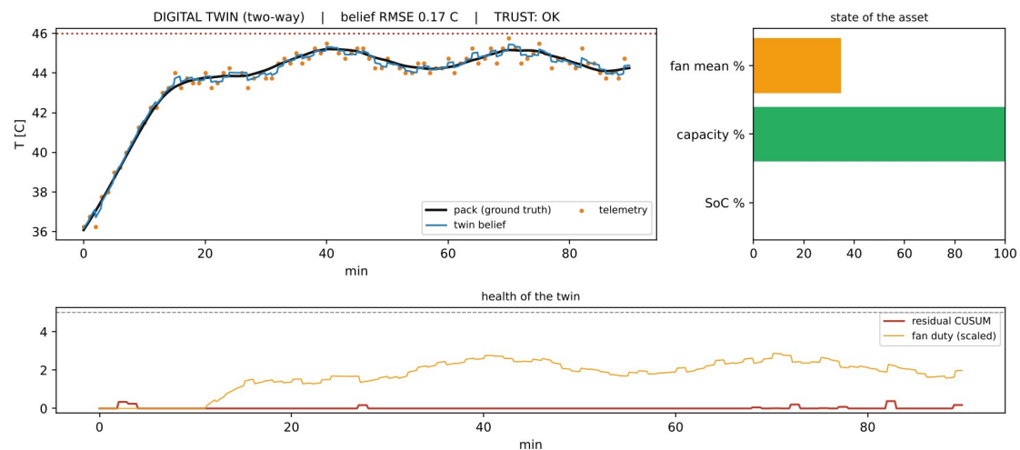
Figure. The dashboard of the twin after a healthy run of 90 minutes: temperature with its limit, the state of the asset, and the cumulative sum of the residuals that carries the trust of the twin.
