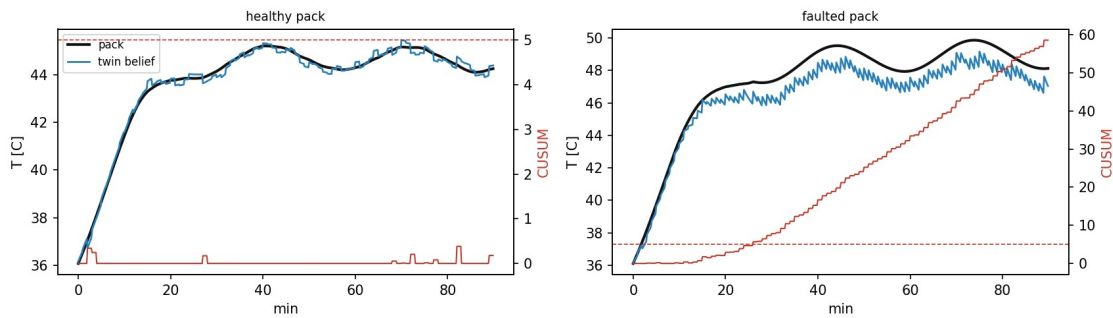
Figure. The assembled twin on the healthy pack, left, and on the faulted pack, right: the pack, the belief of the twin and, on the right axis, the cumulative sum with its decision limit.
