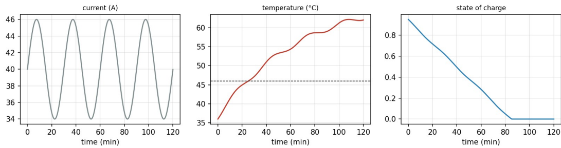
Figure. Two hours of a highway trip at 35 degrees outside: current, temperature and state of charge of the simulated pack without cooling. The dashed line marks the limit of 46 degrees.
