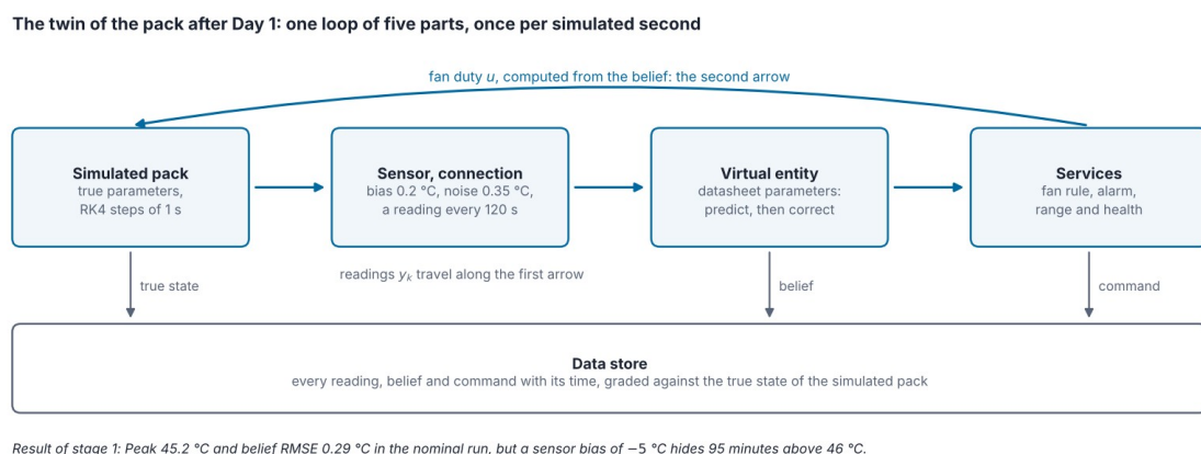
Figure. The twin of the pack after Day 1. The readings travel along the first arrow and the fan duty along the second, and the data store keeps the record against which the twin is graded.
