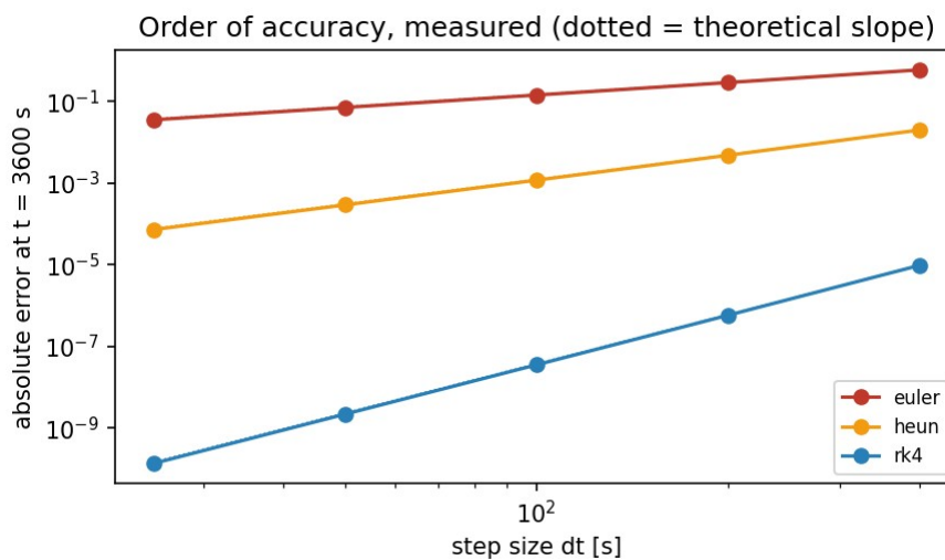
Figure. Error after one hour against the step size, on logarithmic axes. The slopes of the three lines are the orders of the methods. The five points of each line belong to the steps 25, 50, 100, 200 and 400 s, and the dotted lines of the exact slopes 1, 2 and 4 lie hidden under the measured lines.
