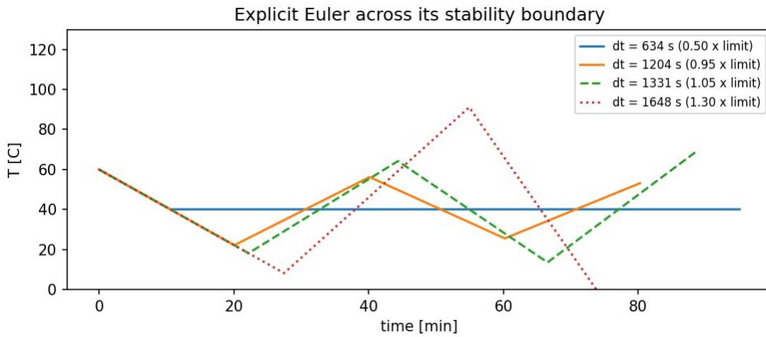
Figure. Explicit Euler at full fan and a constant current of 40 A, started at 60 °C, with steps of 0.5, 0.95, 1.05 and 1.3 times the stability limit.
