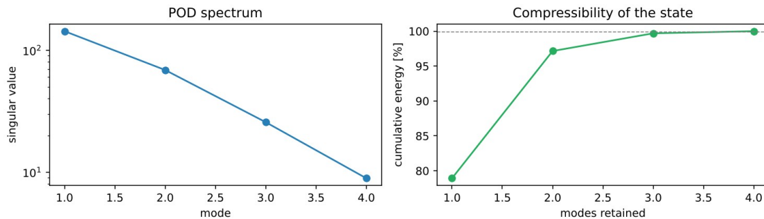
Figure. Left: The four singular values of the snapshots of the pack model, the POD spectrum. Right: The cumulative energy of the modes. Two modes carry about 97 percent, of a four-state system.
