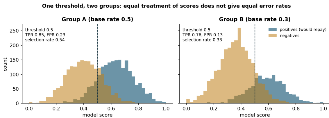
Figure 5.1. Synthetic scores for two groups with different base rates. The same threshold of 0.5 yields different true positive rates, false positive rates and selection rates.
