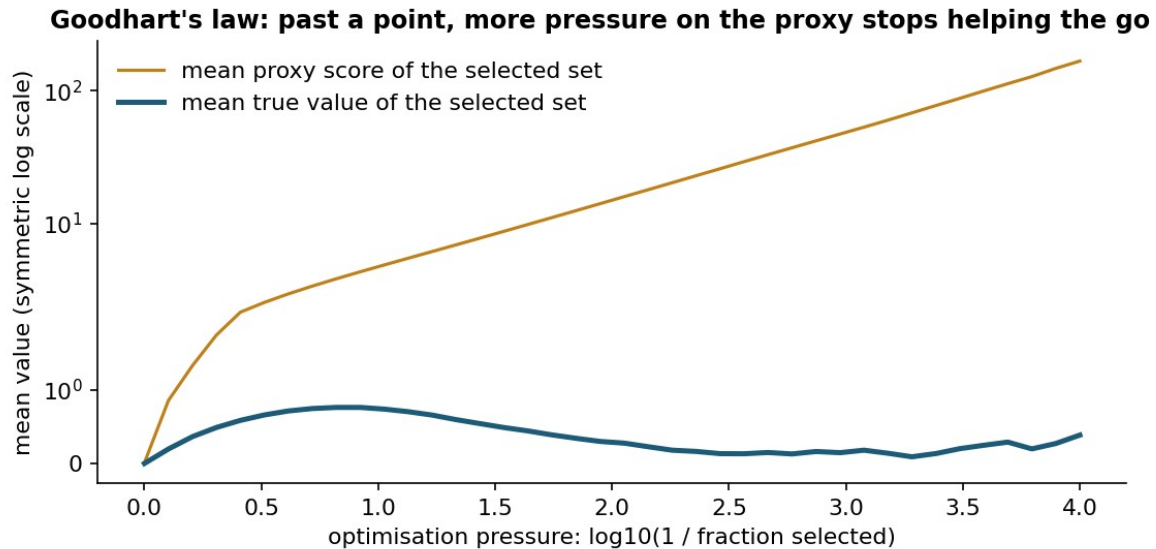
Figure 7.1. Simulated selection on a proxy equal to the true value plus heavy-tailed noise. Moderate selection raises the true value of the chosen items; extreme selection mainly selects noise [2].
