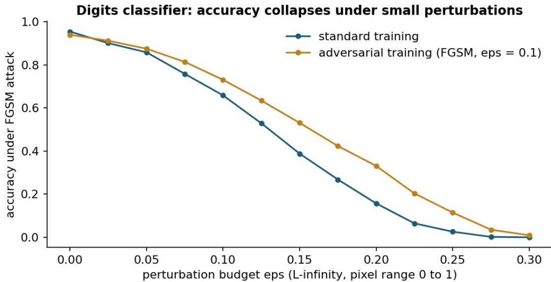
Figure 8.1. Accuracy of a softmax classifier on the digits data set under FGSM attacks of growing budget, with standard and adversarial training [2, 4].
