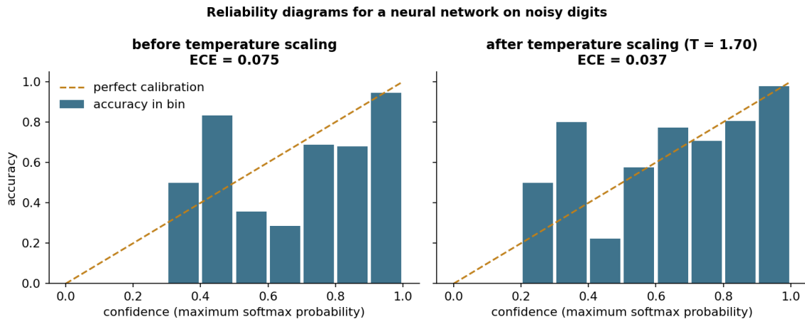
Figure 9.1. Reliability diagrams on a held-out test set before and after temperature scaling for a neural network trained on noisy digits [1].
