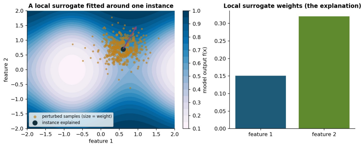
Figure 10.1. A local surrogate explanation. Perturbed samples near the instance are weighted by proximity, and a weighted linear model fitted to the model's outputs gives the local feature weights [5].
