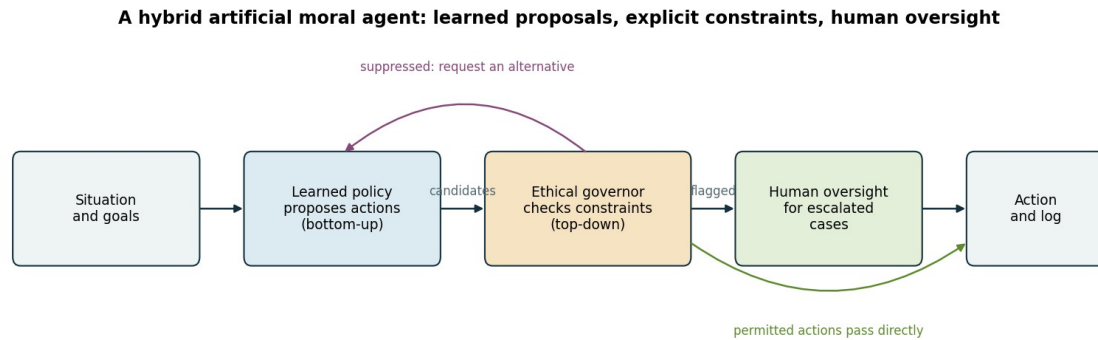
Figure 3.1. A hybrid artificial moral agent. A learned policy proposes actions, an ethical governor removes those that violate constraints, and flagged cases are escalated to a human [3, 5].
