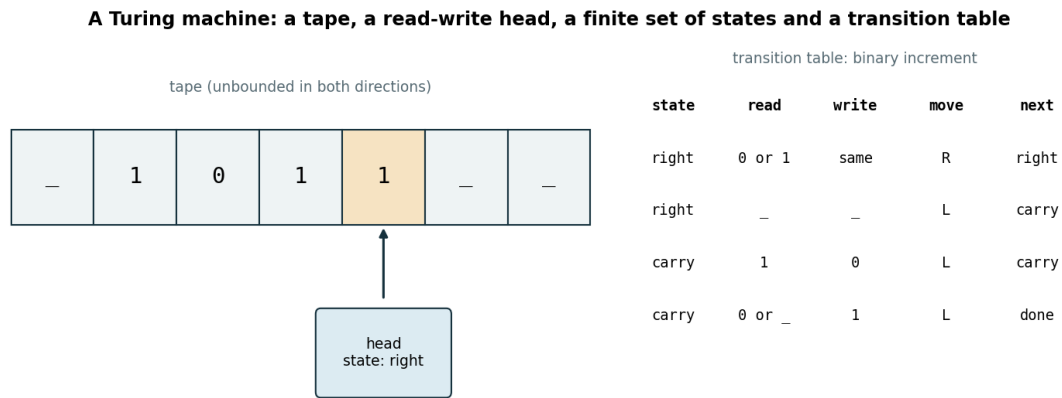
Figure 3.1. A Turing machine for adding one to a binary number: the head moves to the right end, then propagates the carry to the left [1].
